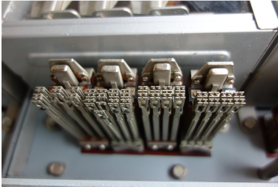
Figure 1: computer
